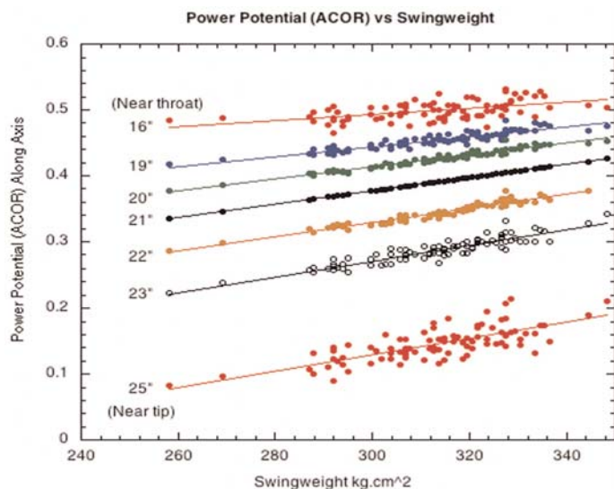
Figure 1. Power Potential vs Swingweight.
